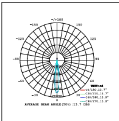
20W CRI90 15°
